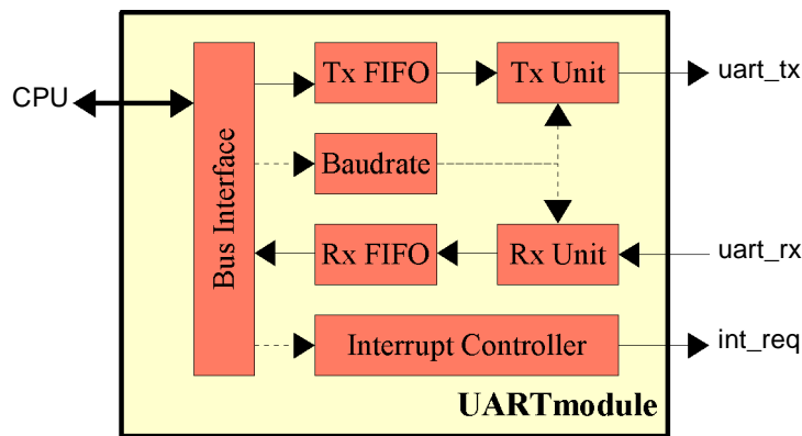
Figure 1: Block diagram
